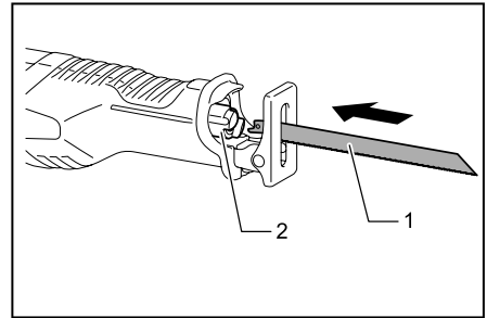
► 1. Reciprocating saw blade 2. Blade clamp sleeve
