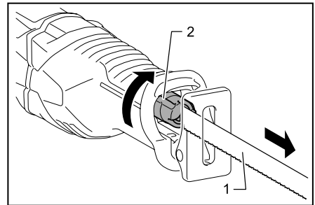
► 1. Reciprocating saw blade 2. Blade clamp lever
