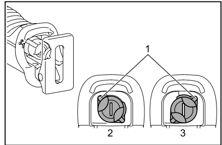
► 1. Blade clamp lever 2. Released position 3. Fixed position
